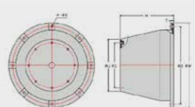
SUPER CONE RUBBER FENDERS
