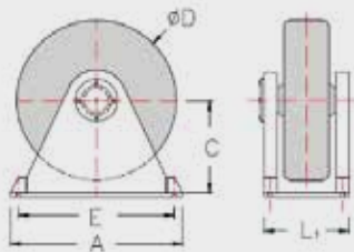
ROLLER FENDERS
