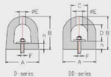
D - FENDERS
