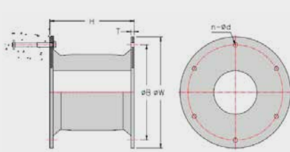
SUPER CELL RUBBER FENDERS
