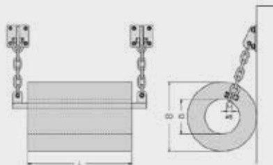
CYLINDRICAL RUBBER FENDERS
